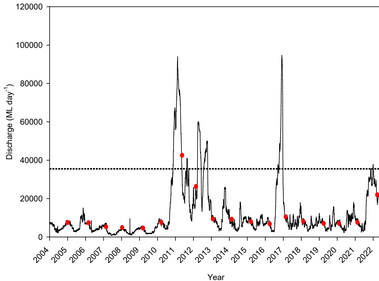
Figure 3. Mean daily flow (ML.d -1 ) in the River Murray at the South Australian Border (Site A42610010) January 2004–June 2022 (MDBA, unpublished data). Closed red circles indicate sampling events and the dotted line represents approximate bankfull discharge at Chowilla (~35,000 ML.d -1 ).
