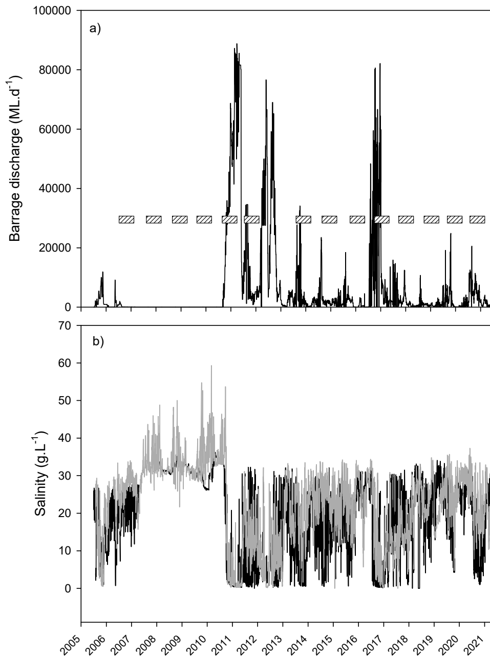
Figure 3-1. a) Mean daily flow (ML.d -1 ) to the Coorong through the Murray Barrages (all barrages combined) from July 2005–June 2021 and b) Mean daily salinity (g.L -1 ) of the Coorong below Tauwitchere (grey line) and Goolwa (black line) barrages from July 2005–June 2021. Sampling periods are represented by hatched bars.
