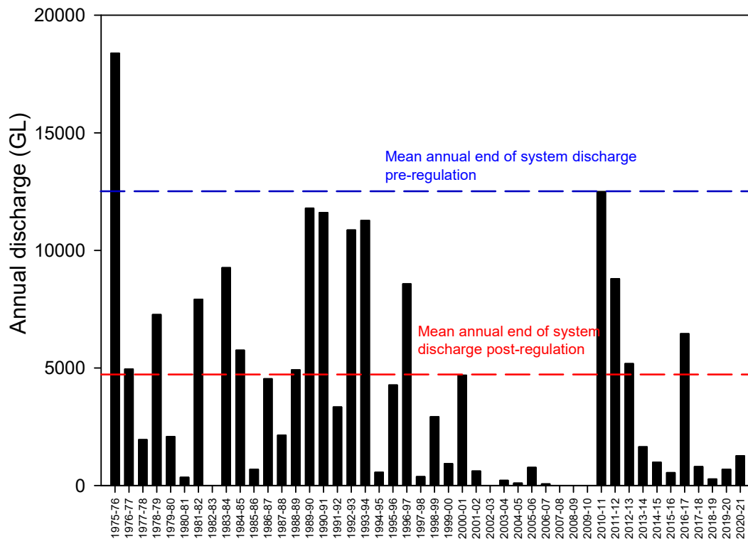
Figure 2-2. Annual freshwater discharge (GL) through the Murray Barrages into the Coorong estuary from 1975–June 2021. Dashed lines represent mean annual end of system discharge pre- (blue) and post-regulation (red).
